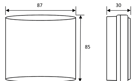
fig. 2. Dimensions (mm)
